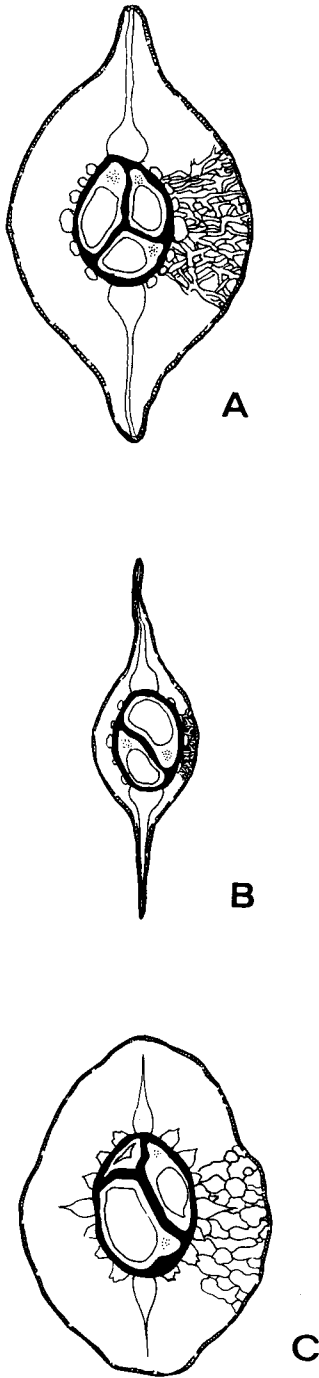
Figure 2: T.S. of mature fruits of A. Bencomia caudata , B, Marcetella moquiniana and C. M. maderensis showing the fleshy/spongy nature of the receptacle in all three (sp = spongy tissue).
